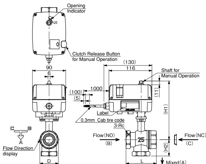
Three-way Valve
