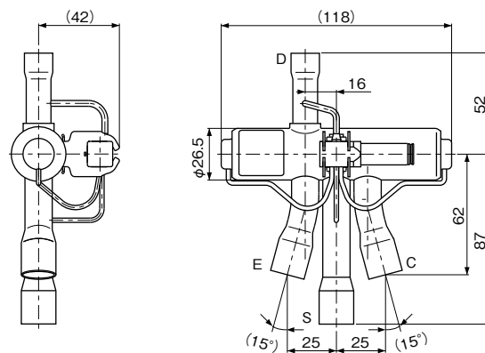
Type STF-H0301
