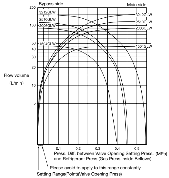
Type SWR
