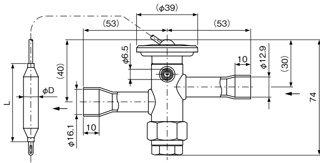
Type SCX-45D
