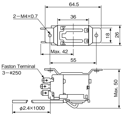
Type HTB
