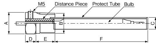
Protect Tube
