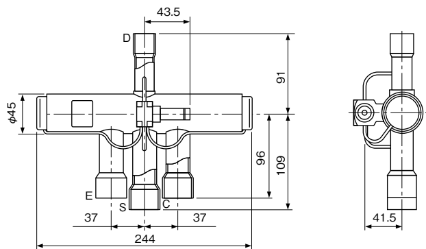
Type STF-2011G
