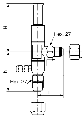
Type EPR-B
