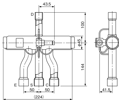
Type STF-2501G
