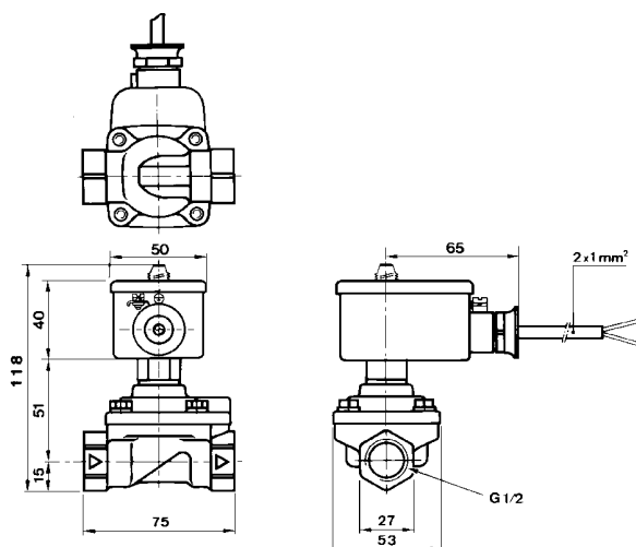
Dimension reference 75
