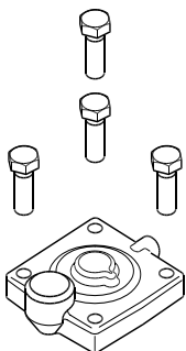
Fig. 3 - Blank top cover ICM 25-65
