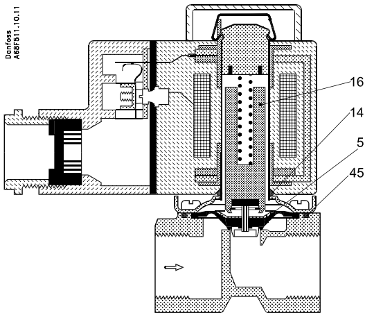
Fig. 1 EVSR 10, 12, 14, 18, 22
