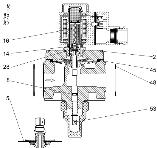
Fig. 1, EVRAT 20 (NC) with plug-in armature tube assembly
