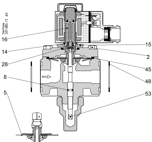
Fig. 1, EVRAT 20 (NC), previous design
