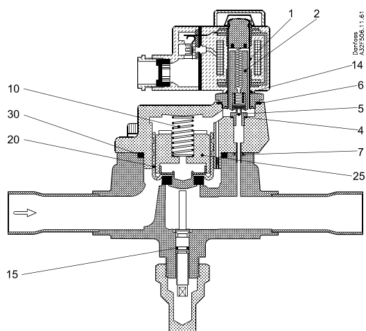
Fig. 1, EVRAT 15 (NC) with plug-in armature tube assembly
