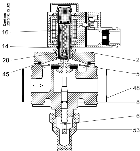
Fig. 1, EVRA 15 (NC) with plug-in armature tube assembly
