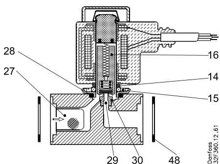
Fig. 1, EVRA 3 (NC), previous design
