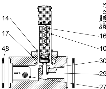
Fig. 2, EVRA 3 (NC) with plug in armature
