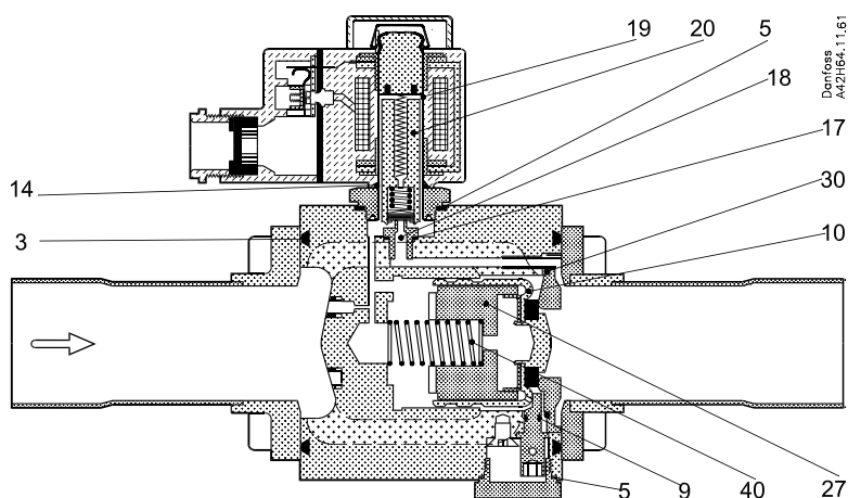
Fig. 1, EVR 40 (NC) with stainless steel piston assembly, previous design
