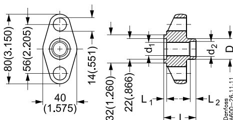
Tongue flange
