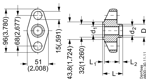
Tongue flange
