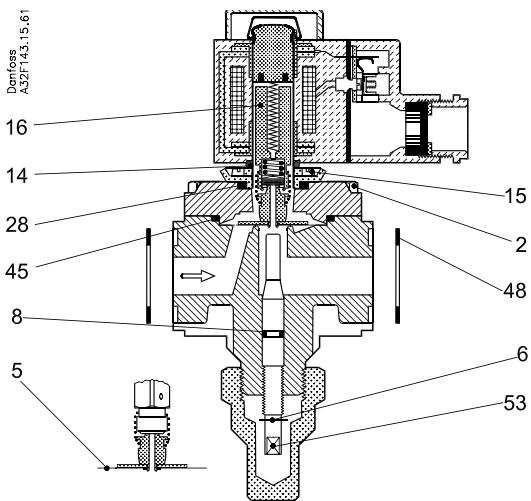
Fig. 1, EVRAT 10 (NC), previous design
