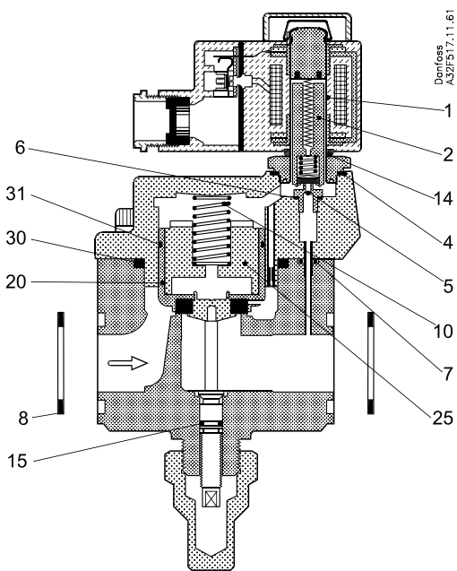
Fig. 1, EVRA 25 (NC) with cast iron piston and piston ring
