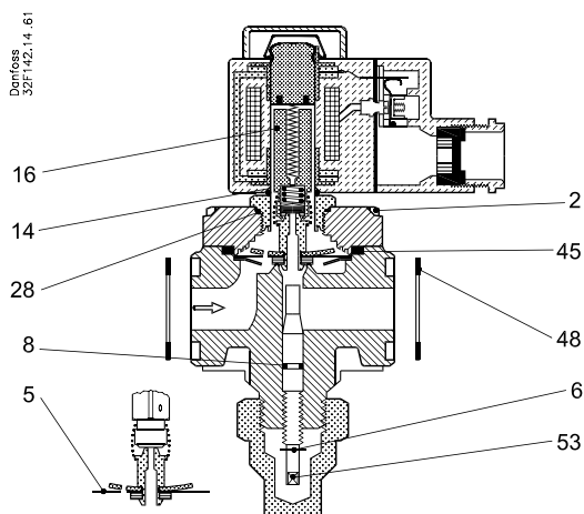
Fig. 1, EVRAT 10 (NC) with plug-in armature tube assembly
