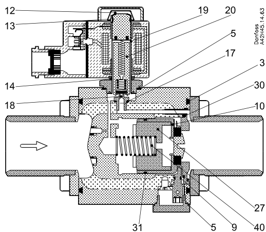
Fig. 1, EVRA 32 and 40 (NC) with cast iron piston and piston ring
