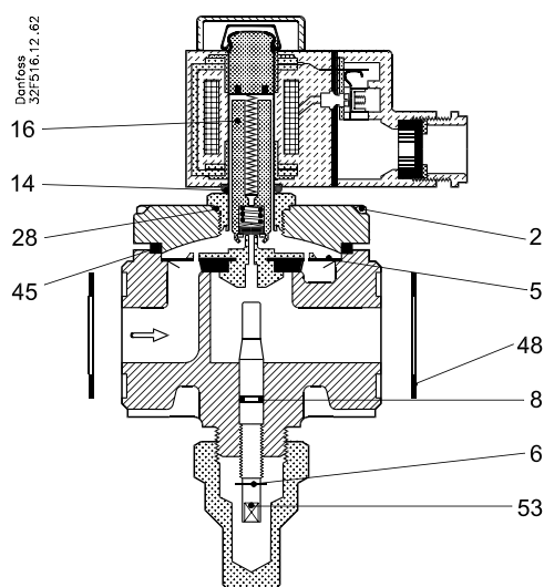
Fig. 1, EVRA 20 (NC) with plug-in armature tube assembly
