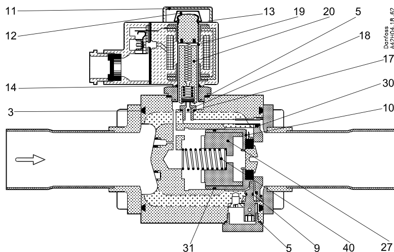
Fig. 1, EVR 40 (NC) with cast iron piston and piston ring
