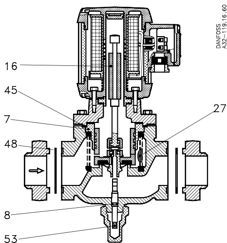
Fig. 1, EVSA 25, 35 and 50
