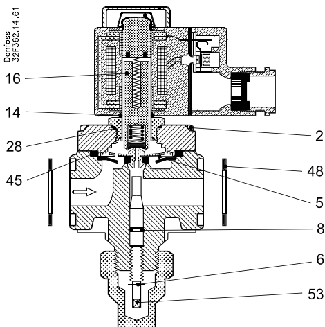
Fig. 1, EVRA 10 (NC) with plug-in armature tube assembly
