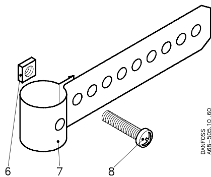
Fig. 3, Bulb strap
